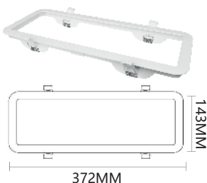
BEAM 3013 (recessed accessory)
