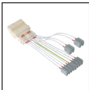
AC input terminal Model No: Beam S0819-5 Beam S0819-8 Beam S0819-11 1 unit required per line
